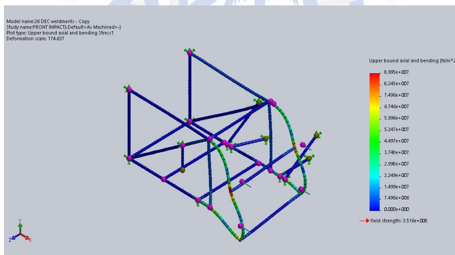
Figure 7.6. FRONT IMPACT-Stress-Stress I
