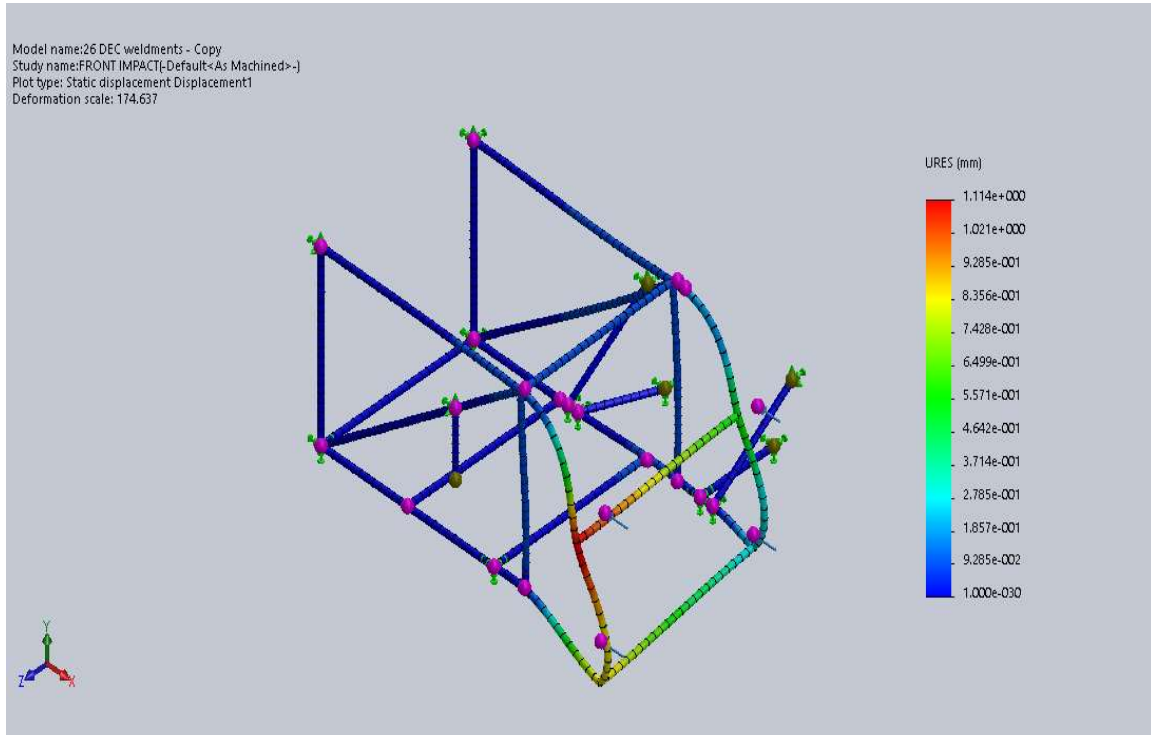
Figure 7.7 FRONT IMPACT-Displacement-Displacement1
