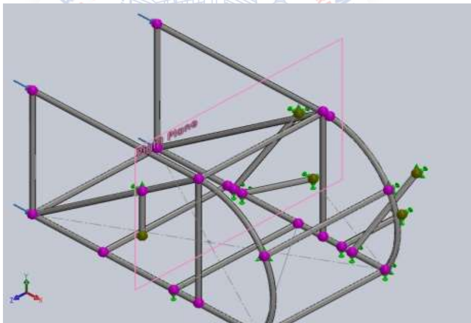
Figure 7.5 Forces applied on model
