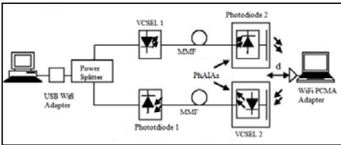
Fig. 6: System Configuration [12]
