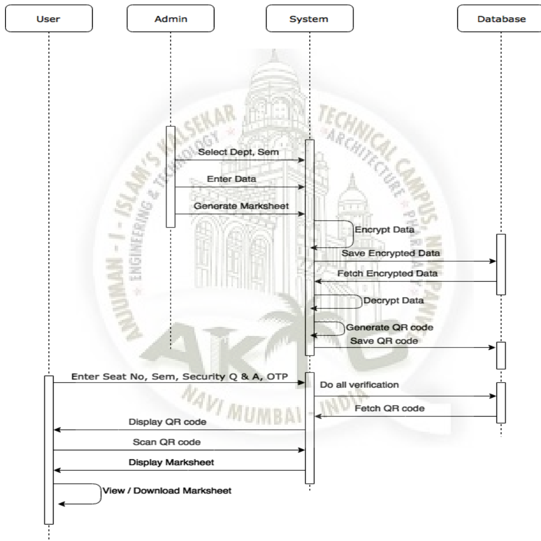
Figure 5.10: Sequence Diagram
