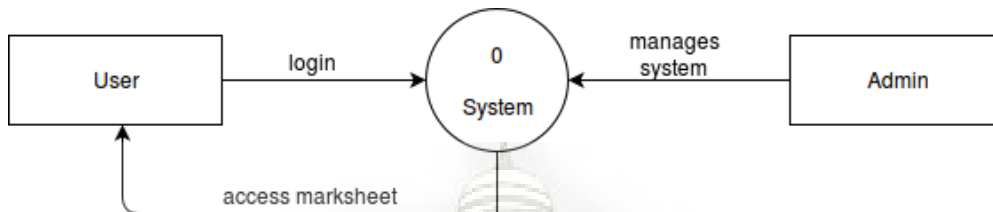
Figure 5.3: DFD Level 0
