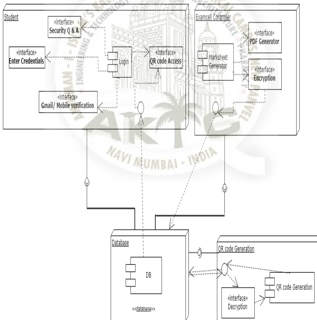
Figure 5.11: Component Diagram
