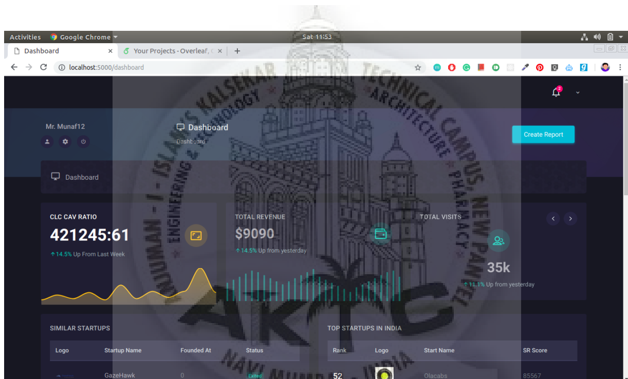
Figure 6.1: User Dashboard
