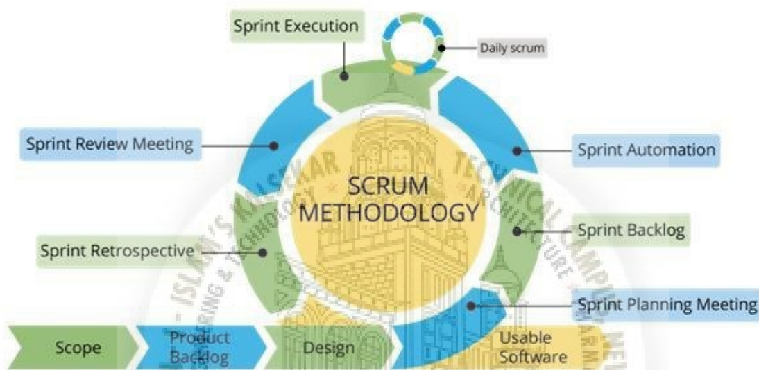
Figure 3.1: Scrum Model
