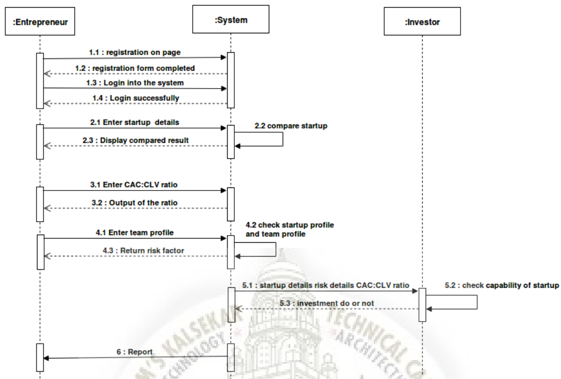
Figure 5.7: Sequence Diagram
