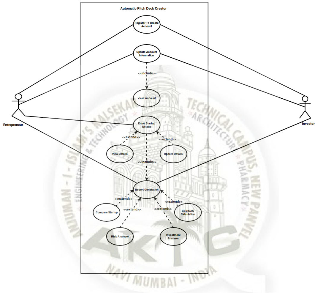
Figure 5.1: Usecase Diagram
