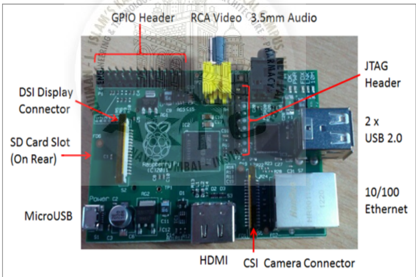
Fig. 4.1: Raspberry pi 3 model B
