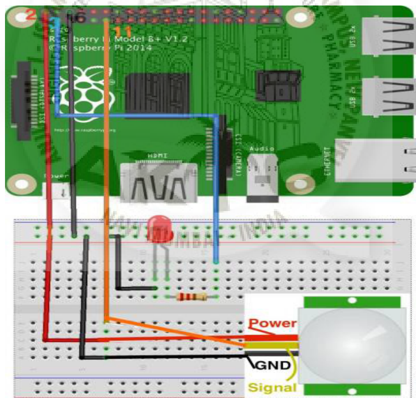
Fig. 4.7: Raspberry pi PIR motion sensor connection
