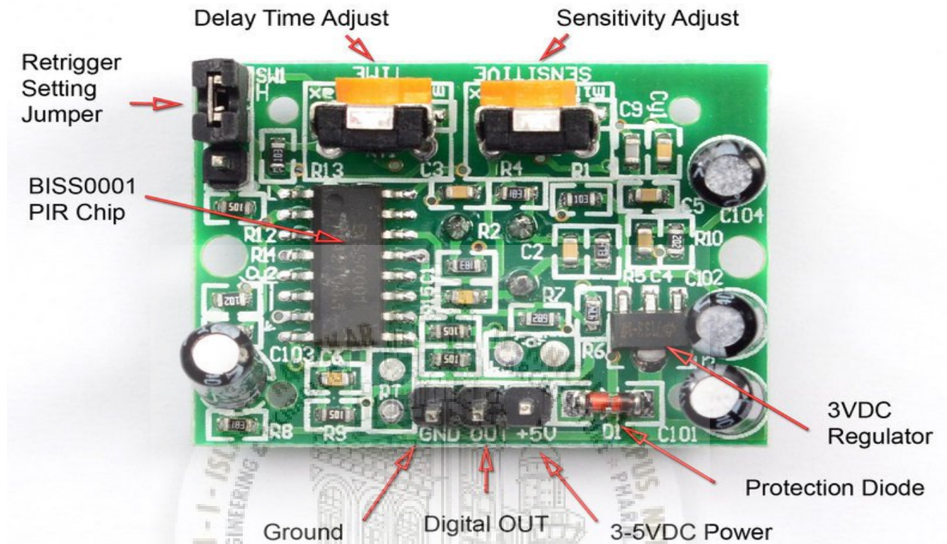
Fig. 4.2: Top View of PIR Sensor
