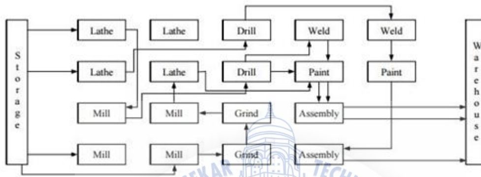
Fig. 5.2 process layout
