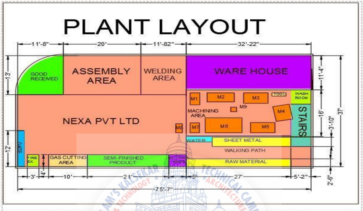
Fig 4.4 Existing Layout
