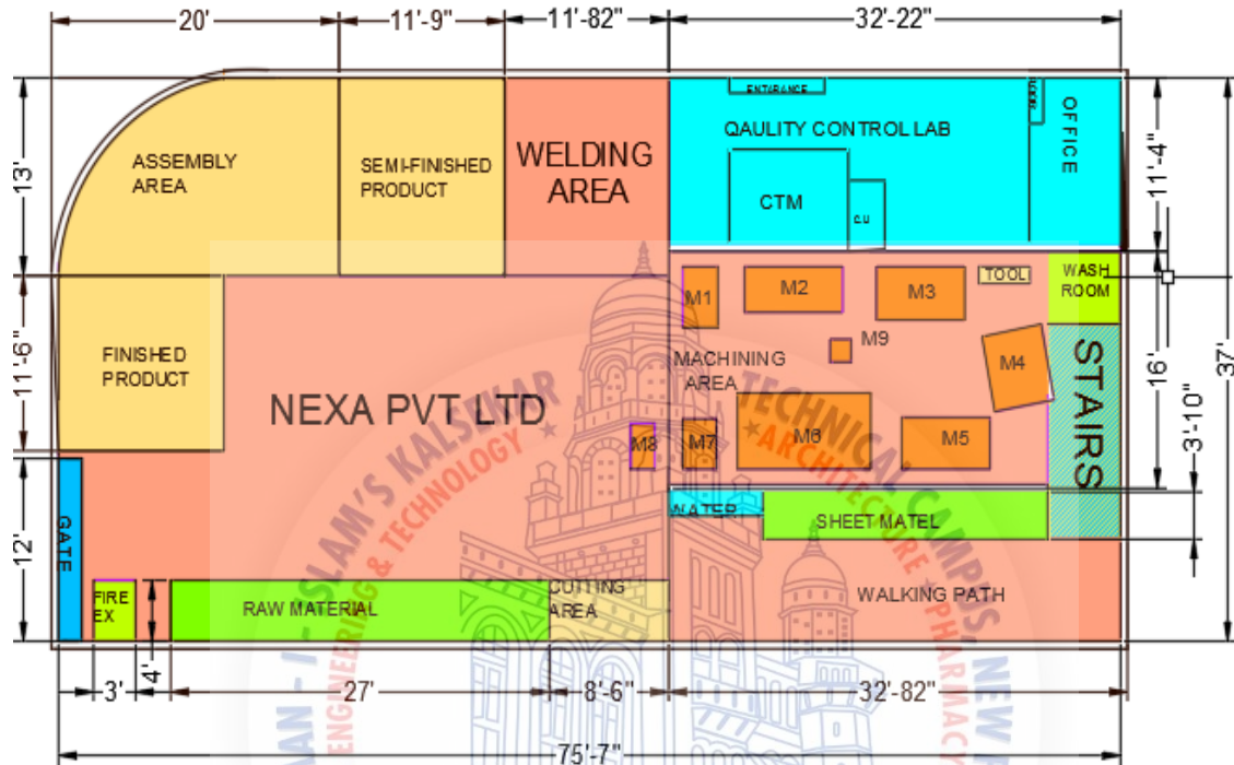
Fig.4.6 Develop Plant Layout
