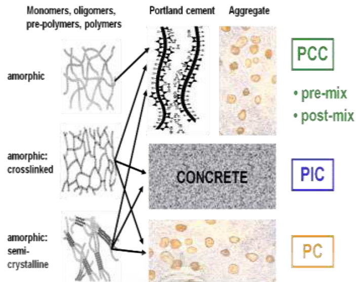
fig no. 2.1 Polymer Concrete Composite
