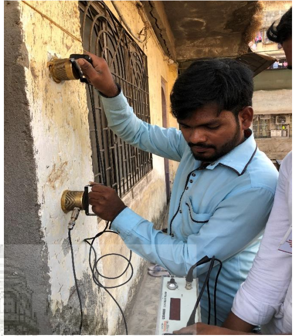
fig no. 5.8 USPV application on exterior columns
