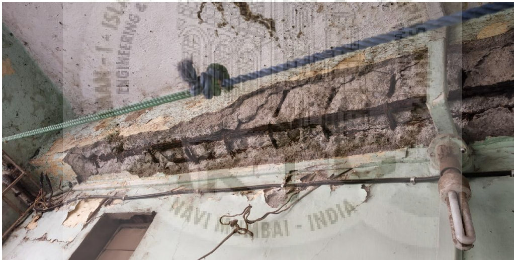
fig no. 5.3 Beam of B-2, Balcony
