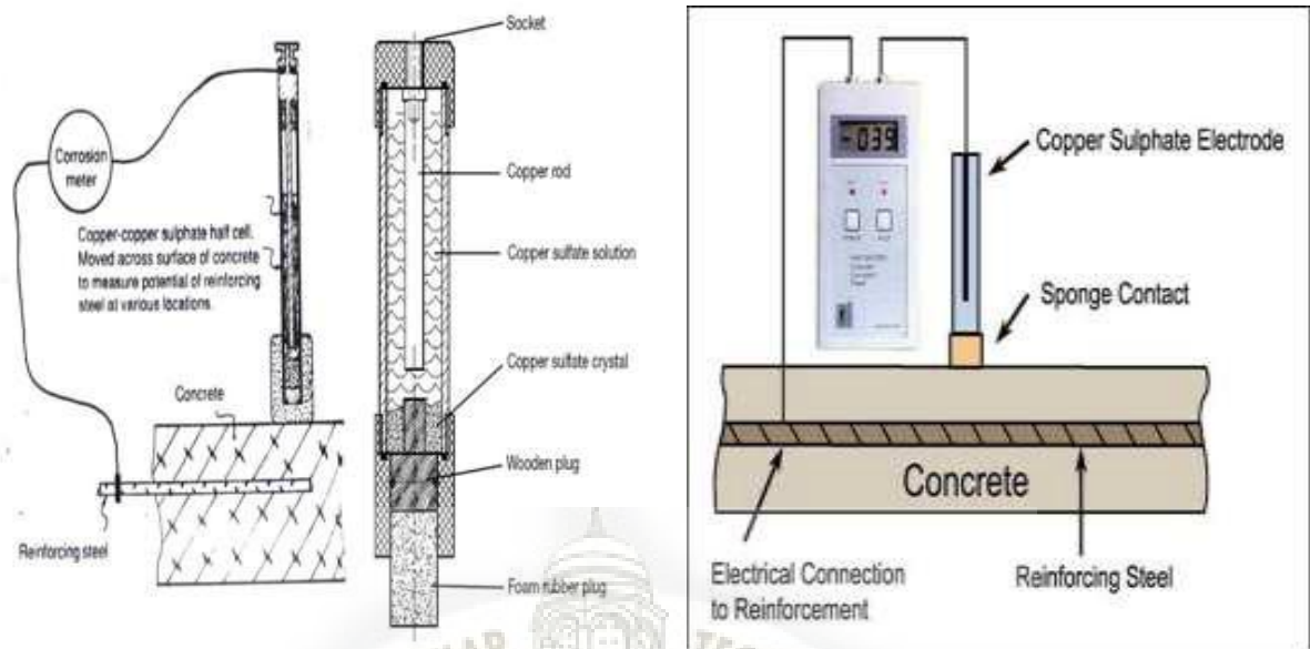
fig no. 1.6 Half cell potentiometer
